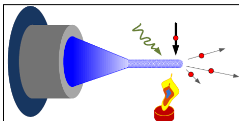
Figure 2: Electron emission from nanotubes can be induced by heating them or illuminating them with photons or other electrons.
