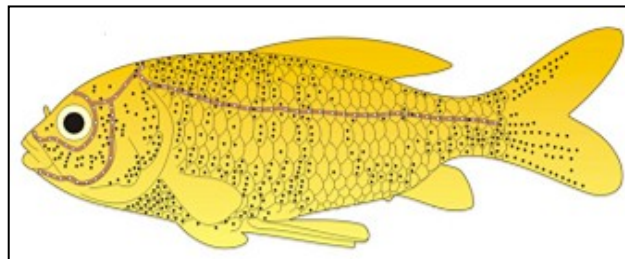
Figure 3. The lateral line and the neuromasts of fish [13]. Black dots indicate position of neuromasts on the skin surface, while white dots on the thick brown line show the approximate positions of neuromasts in sub epidermal lateral line canals.
